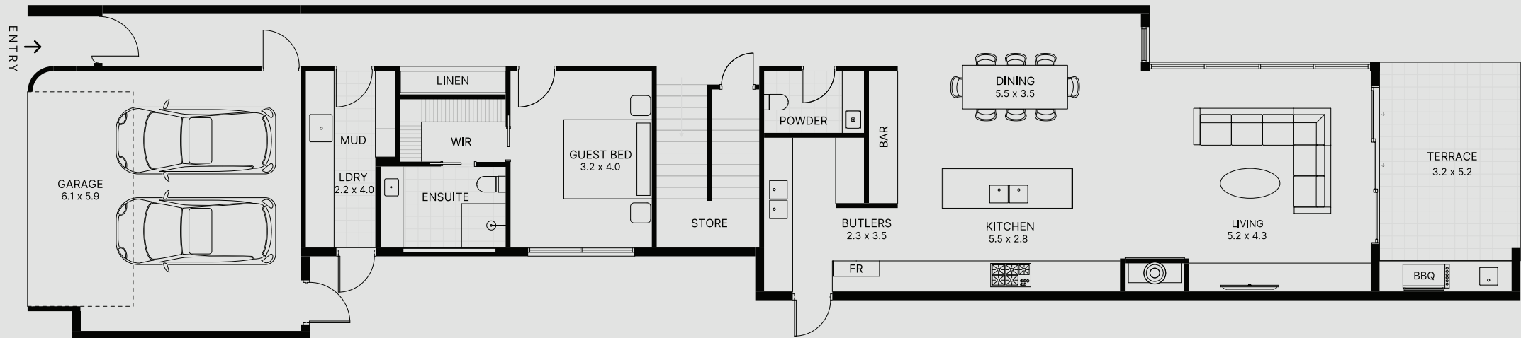
GROUND FLOOR
