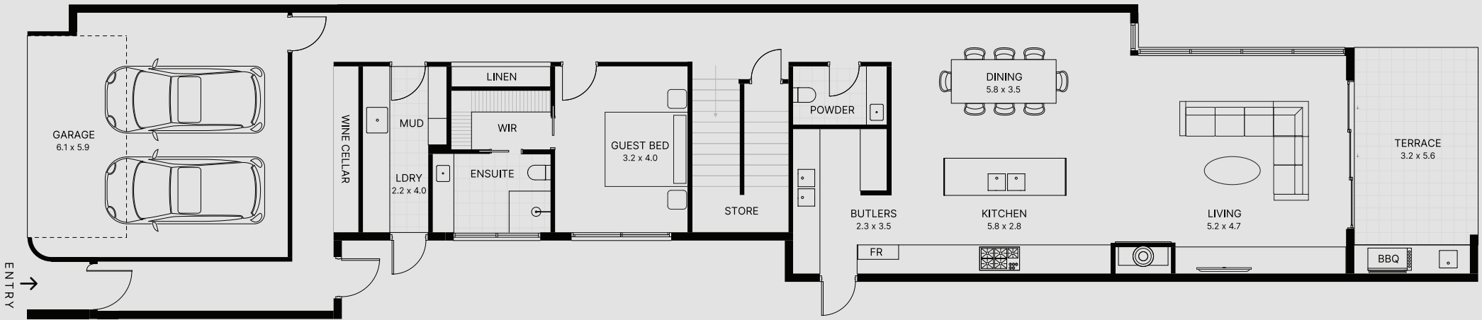
GROUND FLOOR
