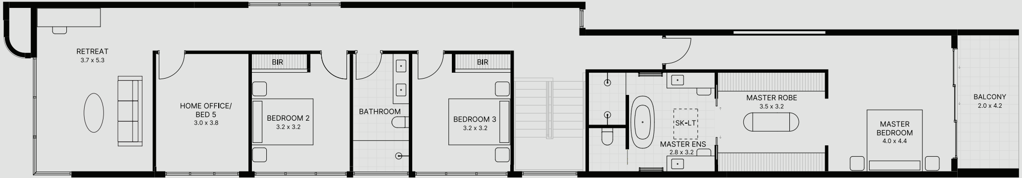
FIRST FLOOR
